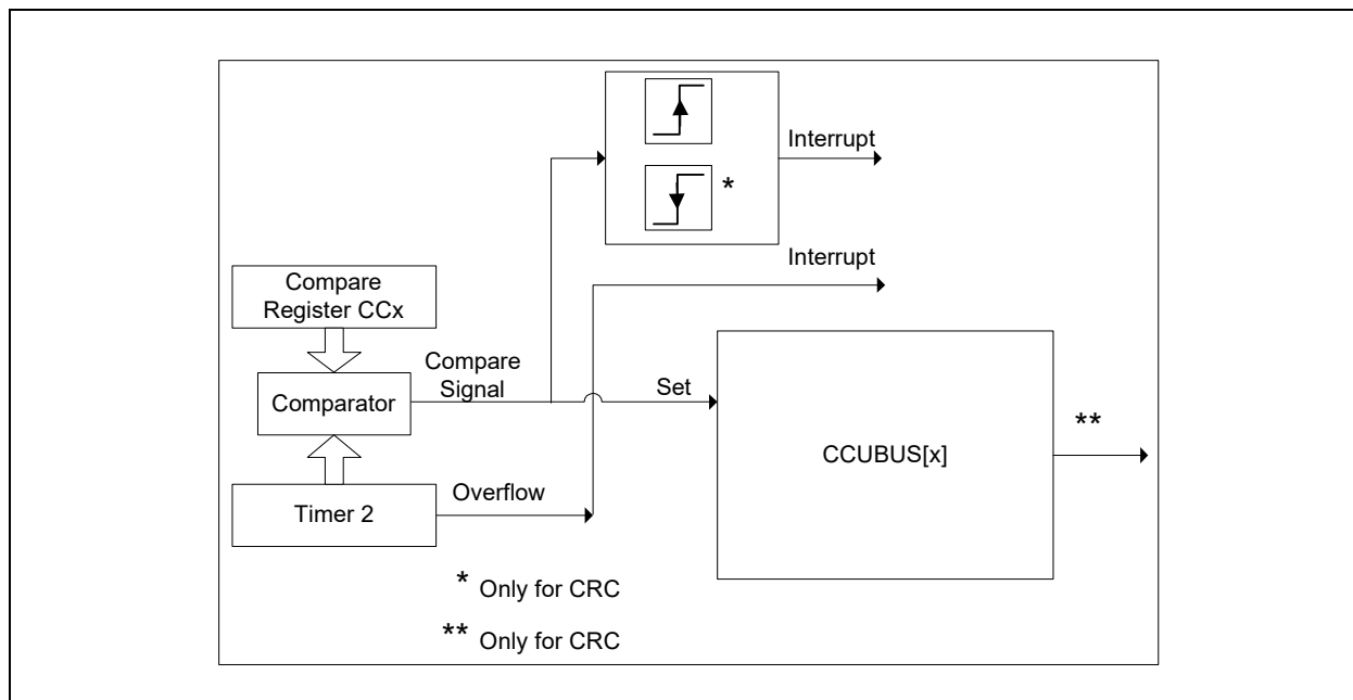
FIGURE 19-9: TIMER 2 IN COMPARE MODE 1
