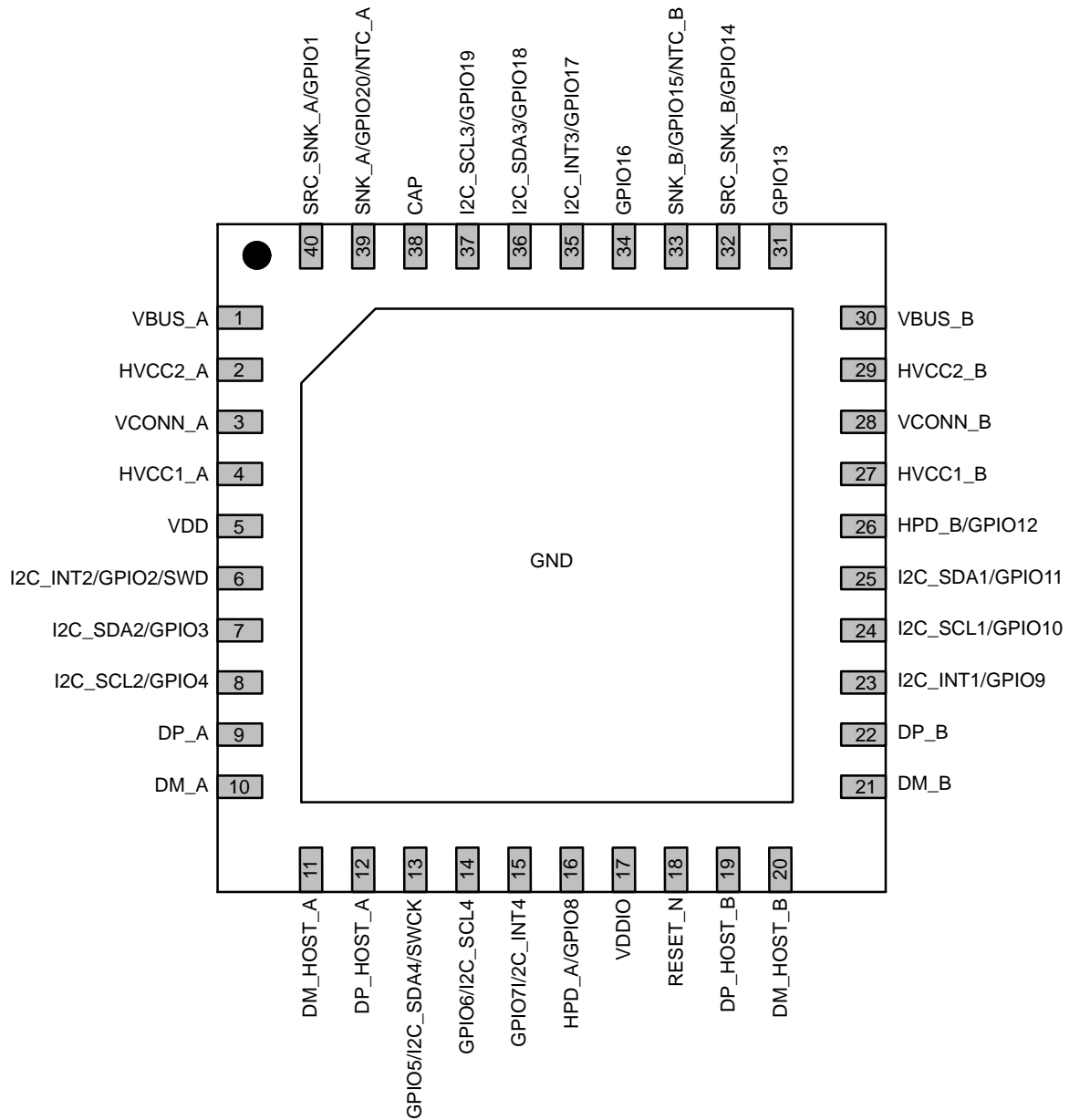
Figure 2. Pin Diagram
