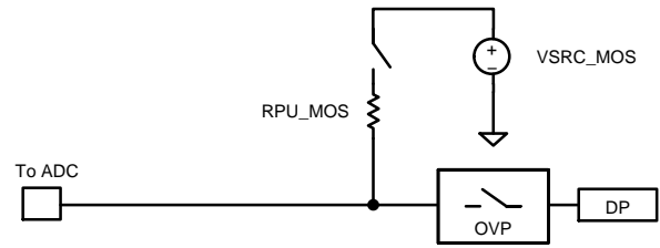
Figure 6. Moisture Detection
