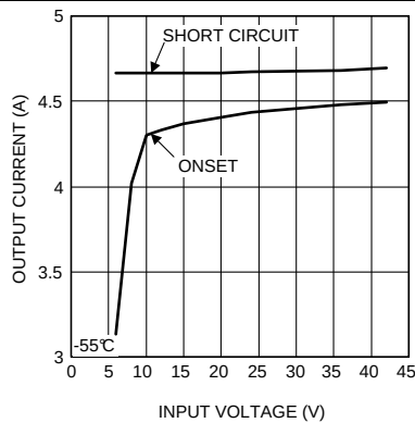
Figure 27. Current Limit 3.3 V_{OUT} at -55^\circ\text{C}
