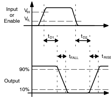
Figure 9. Inverting
