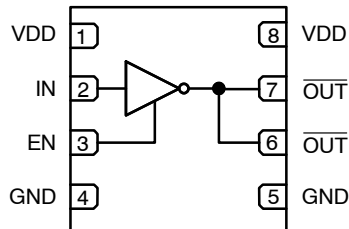
Figure 5. FAN3121 Pin Assignments (Repeated)
