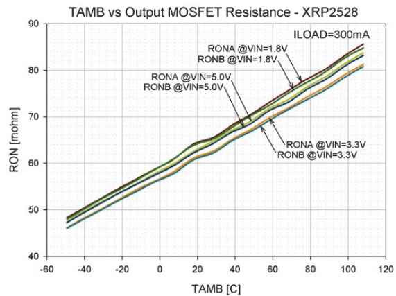
Fig. 5: Output On-Resistance vs. Temperature (XRP2528)
