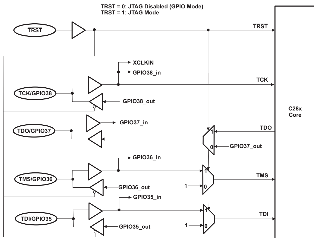
Figure 6-25. JTAG/GPIO Multiplexing
