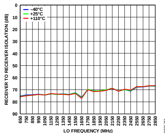
Figure 99. Receiver to Receiver Isolation (dB) vs. LO Frequency (MHz)
