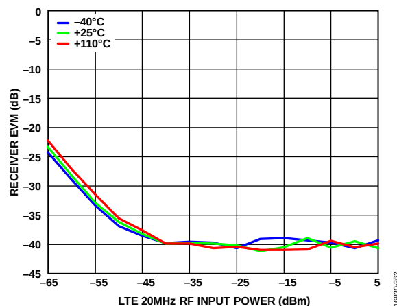
Figure 98. Receiver EVM vs. LTE 20 MHz RF Input Power, LTE 20 MHz RF Signal, LO = 2700 MHz
