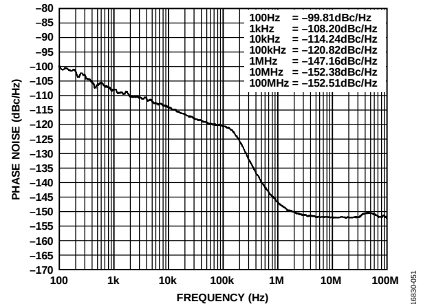
Figure 51. LO Phase Noise vs. Frequency Offset, LO = 300 MHz, PLL Loop Bandwidth = 50 kHz
