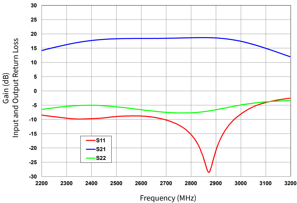
Figure 4. Small Signal Gain and Return Losses vs Frequency V_{DD} = 28\text{ V} , I_{DQ} = 0.13\text{ A}
