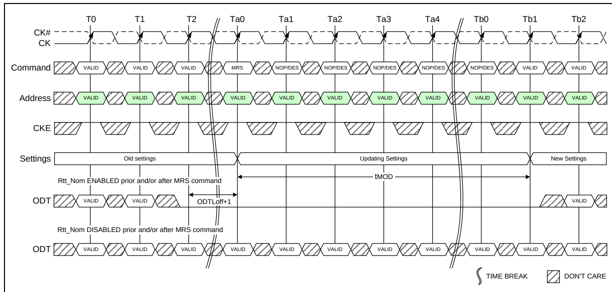
Figure 4 – t_{MOD} Timing
