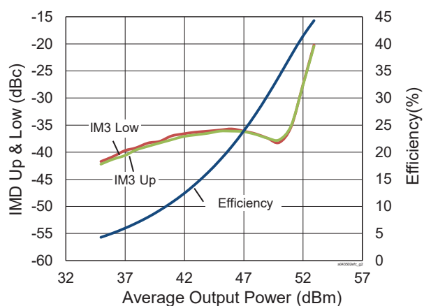
Two Tone Drive-up V_{DD} = 50 \text{ V} , I_{DQ} = 850 \text{ mA} , f = 860 \text{ MHz} , 1 MHz Tone Spacing
