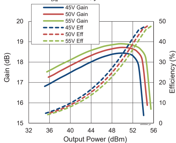
CW Performance at various V_{DD} I_{DQ} = 850 \text{ mA} , f = 860 \text{ MHz}
