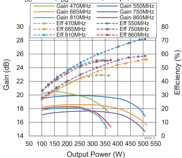
Pulsed RF Performance V_{DD} = 50 \text{ V} , I_{DQ} = 850 \text{ mA} , 100 \mu\text{s} , 10% DC
