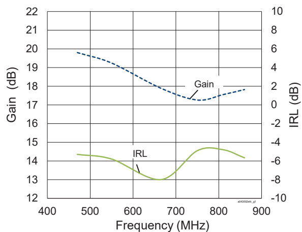
DVB-T Performance Gain & IRL vs Frequency P_{OUT} = 48.5 \text{ dBm} , V_{DD} = 50 \text{ V} , I_{DQ} = 850 \text{ mA}
