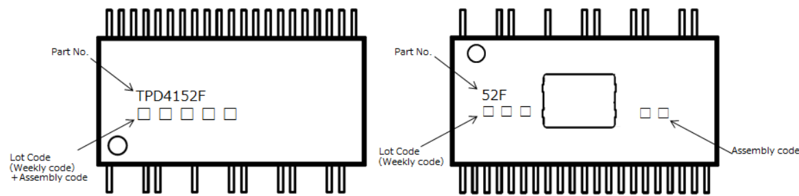
TPD4152F,BF(S)
