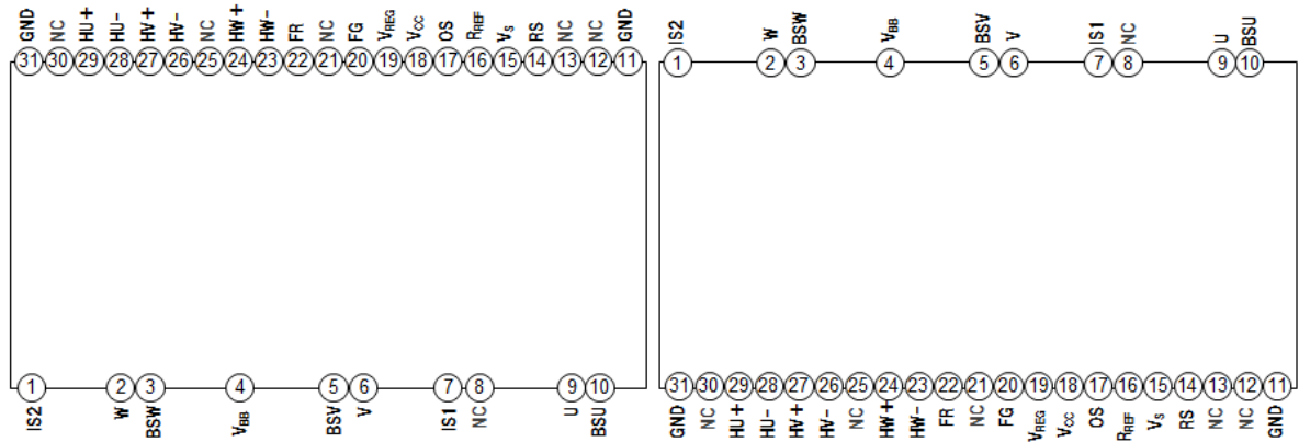
TPD4152F,BF(S)
