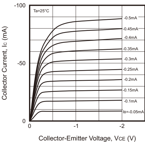
Fig.1 - Static Characteristic
