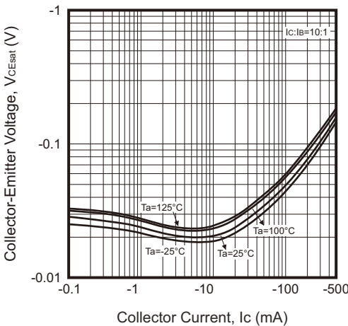
Fig.3 - Collector-Emitter Saturation Voltage
