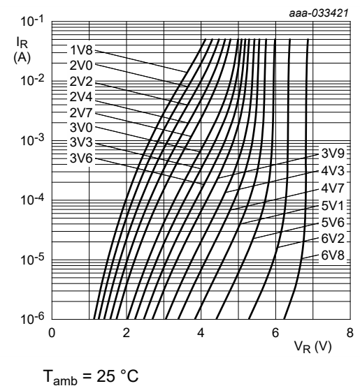
Fig. 5. Reverse current as a function of reverse voltage; typical values (BZX58550-B/C1V8-Q to BZX58550-B/C6V8-Q)
