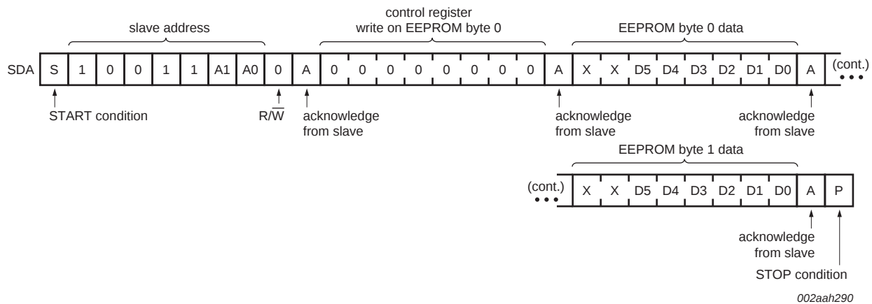
Fig 10. Write on two EEPROMs, assuming WP = 0
