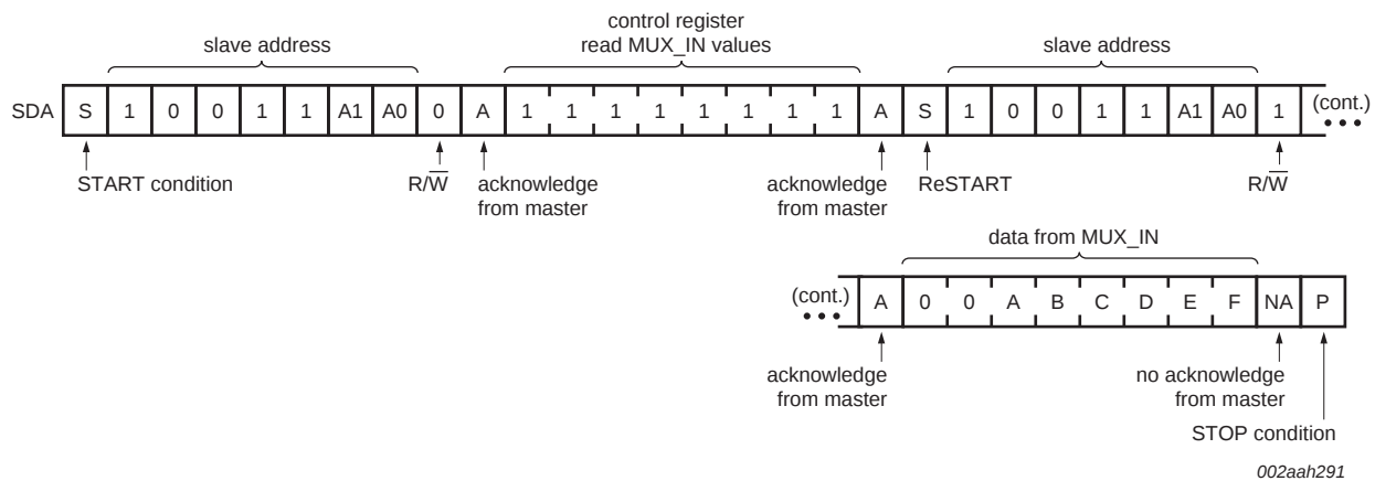
Fig 11. Read MUX_IN register
