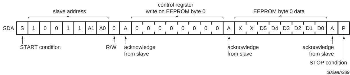
Fig 9. Write on one EEPROM, assuming WP = 0
