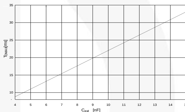
Figure 6: T_{DMAX} as function of external CSSD capacitor
