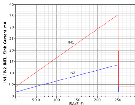
Figure 7: Typical I_{IN1} and I_{IN2} Currents vs R_A The value for R_A can be determined by the formula: R_A = (1.24/I_{RA}) - 750 .
