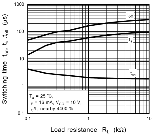
Fig. 11.12 Switching Time - R_L
