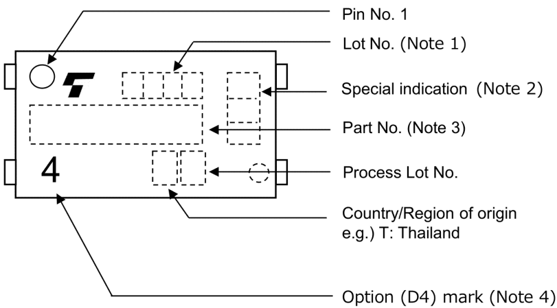
Fig. 15.3 Marking Example
