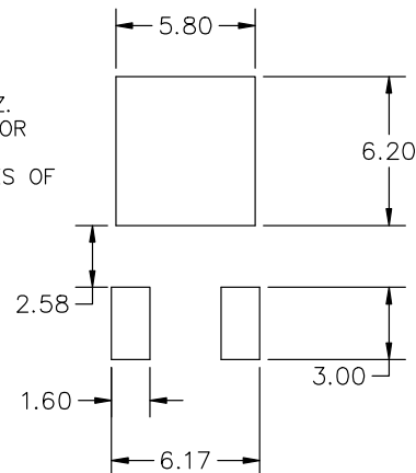
ALTERNATE CONSTRUCTIONS
