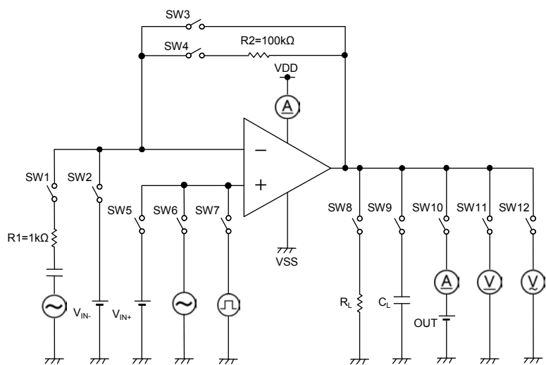
Figure 26. Test circuit 2
