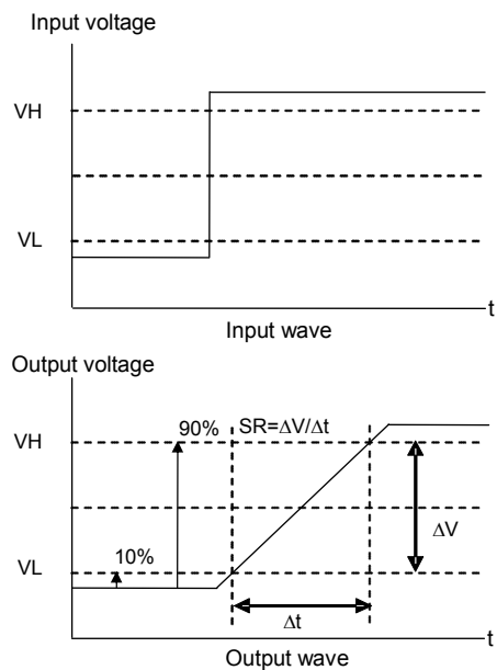
Figure 27. Slew Rate Input and Output Wave
