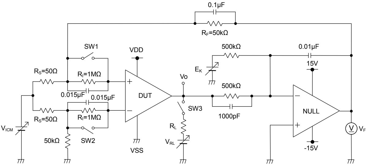
Figure 25. Test circuit 1
