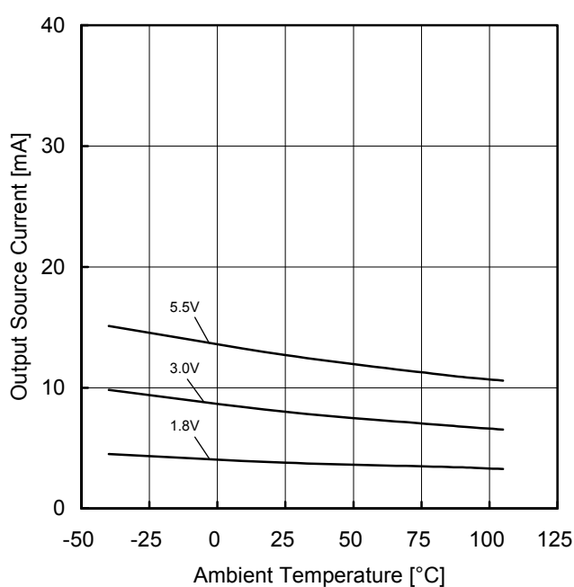
Figure 11. Output Source Current vs Ambient Temperature (OUT=VDD-0.4V)
