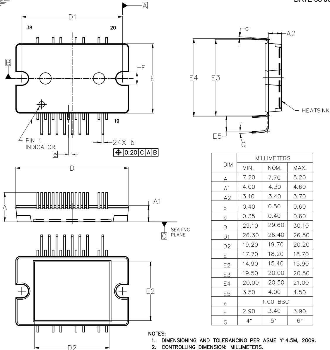
DIP-38, 29.60x18.20x7.70, 1.00P (EP-4) CASE 125BS ISSUE C
