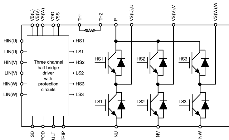
Figure 1. Function Diagram
