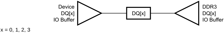
Figure 5-84. DQ[x] Topology
