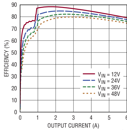
Efficiency vs Output Current V_{OUT} = 8\text{V}
