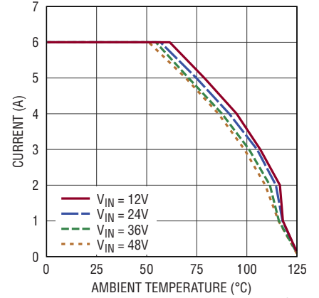
Derating Curve V_{OUT} = 1.8\text{V}
