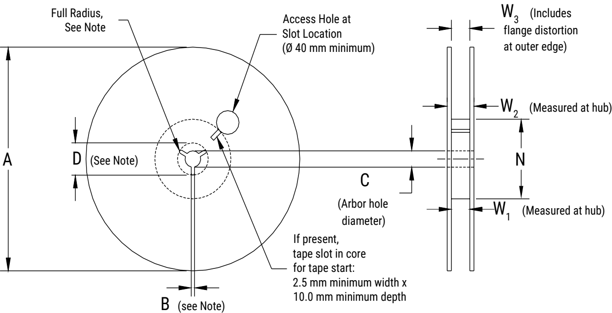
Figure 6 – Reel Dimensions
