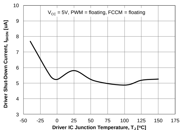
Figure 22. Driver Shutdown Current vs. Temperature
