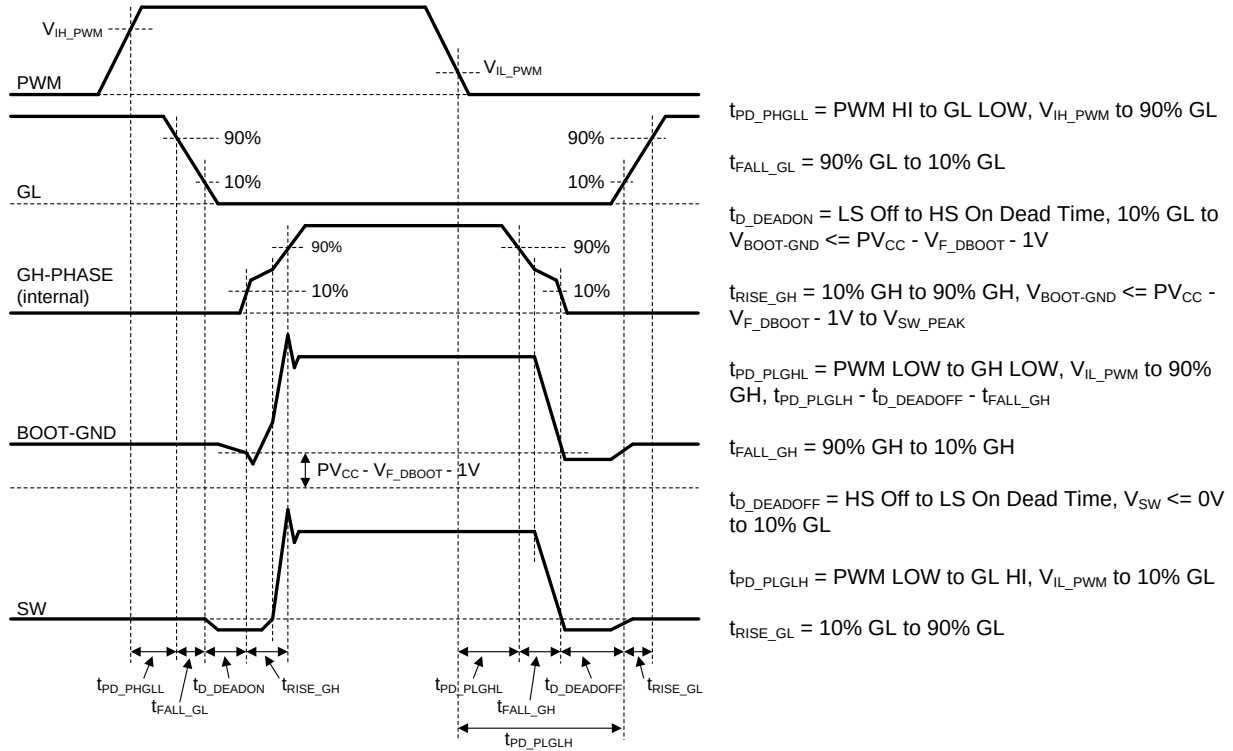
Figure 24. PWM Timing Diagram
