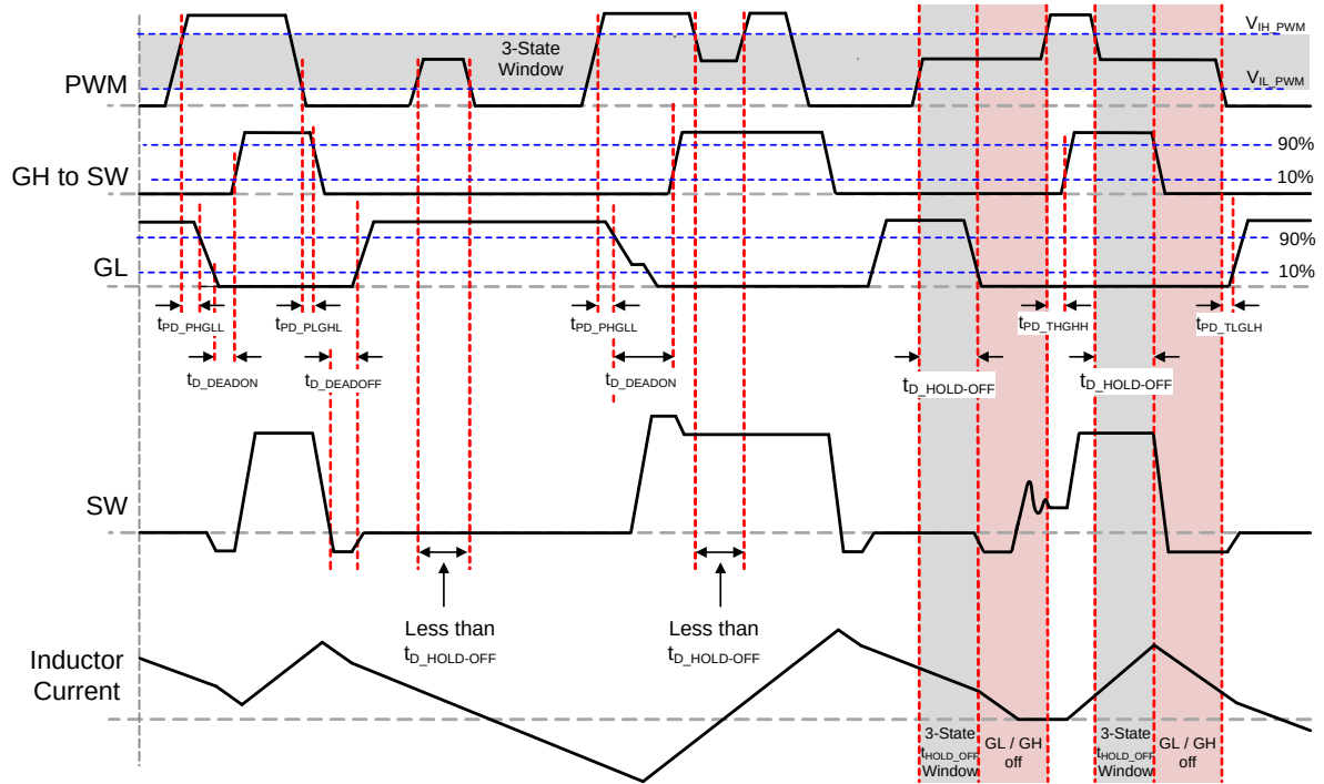
Figure 27. PWM 3-State Timing Diagram (FCCM held HIGH)
