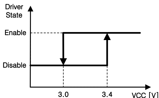
Figure 26. UVLO
