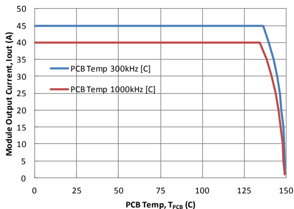
Figure 4. Safe Operating Area with 12 V_{IN}
