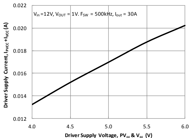
Figure 13. Driver Supply Current vs. Driver Supply Voltage
