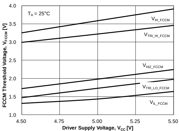
Figure 18. FCCM Threshold vs. Driver Supply Voltage
