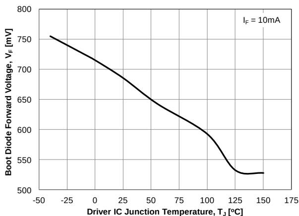
Figure 21. Boot Diode Forward Voltage vs. Temperature
