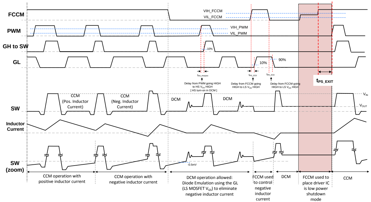
Figure 28. FCCM 3-State Timing Diagram
