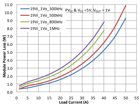
Figure 7. Power Loss vs. Output Current with 19 V_{IN}
