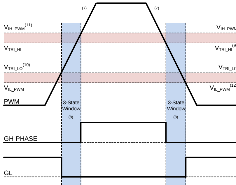
Figure 25. PWM Threshold Definition
