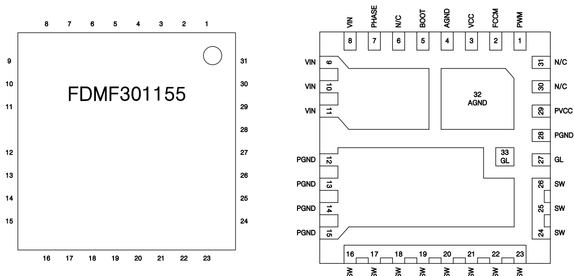
Figure 3. Pin Configuration - Top View and Transparent View
