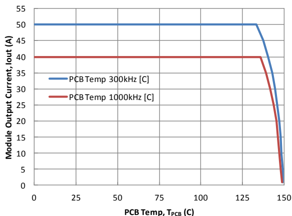
Figure 5. Safe Operating Area with 19 V_{IN}
