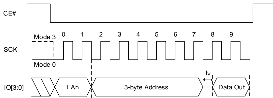
Figure 8.76 Read DVB Sequence In QPI Mode (FAh)
