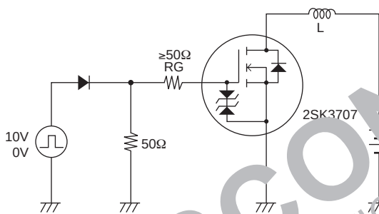
Fig.1 Avalanche Resistance Test Circuit
