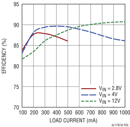
Figure 3. Efficiency Curves
