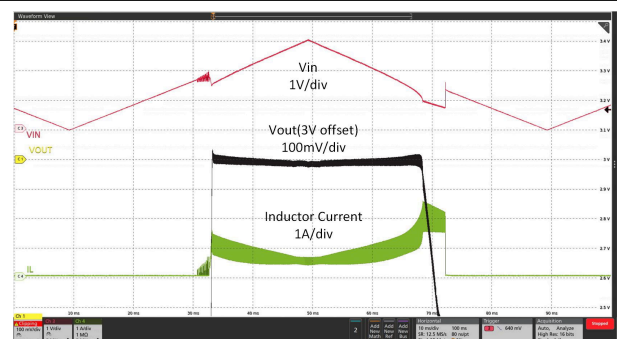
Figure 8-10. Line Transient
