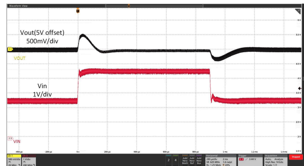
Figure 8-10. Line Transient
