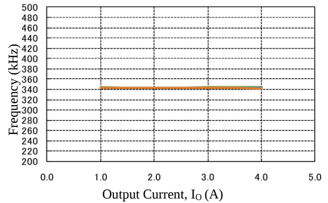
Figure 5-8. Operating Frequency
