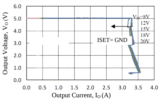
Figure 5-12. Overcurrent Protection
