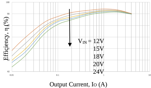
Figure 5-2. Efficiency ( V_O = 5.0 V)
