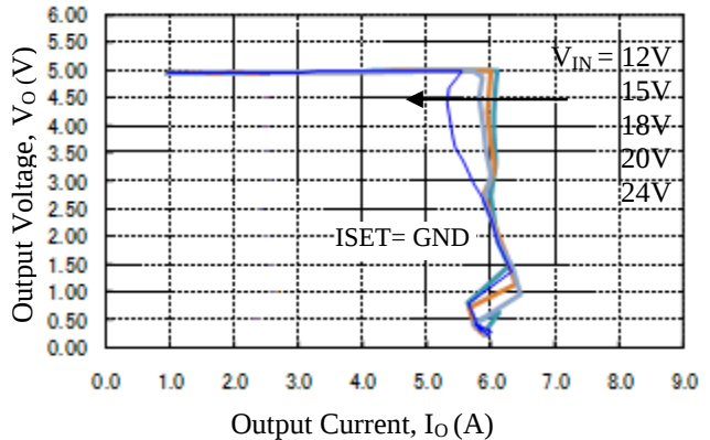
Figure 5-4. Overcurrent Protection
