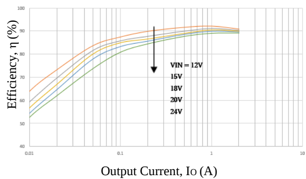
Figure 5-10. Efficiency ( V_O = 5.0\text{ V} )
