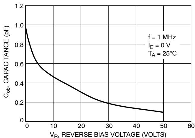
Figure 40. Output Capacitance
