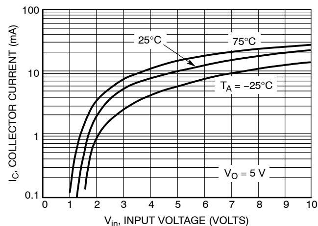
Figure 41. Output Current versus Input Voltage
