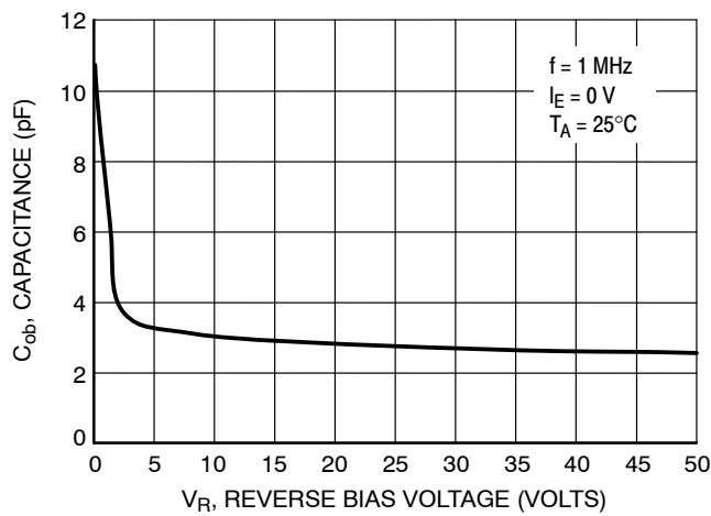
Figure 35. Output Capacitance
