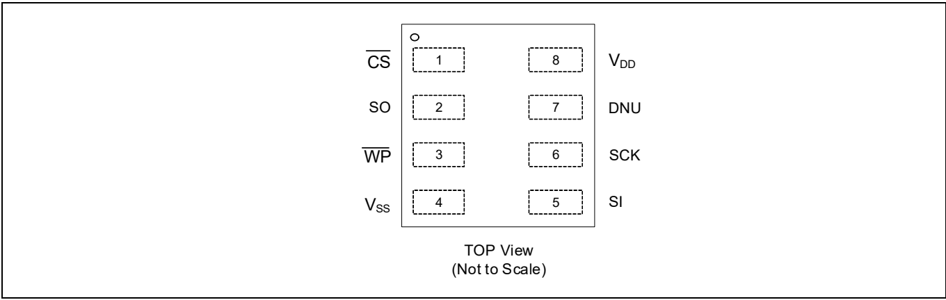
Figure 2 8-pin GQFN/UFLGA pinout
