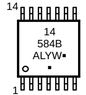
TSSOP-14 DT SUFFIX CASE 948G
