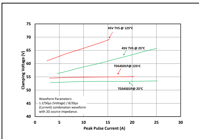
Figure 3- Clamping Comparison
