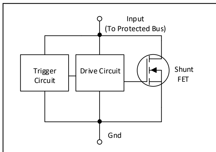
Figure 1- Functional Diagram
