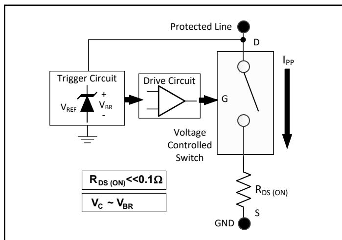
Figure 2- TDS Operation
