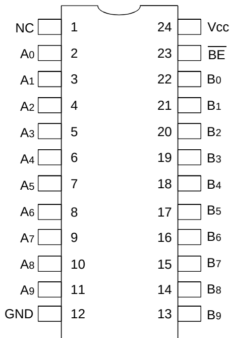
SOIC/ QSOP/ TSSOP TOP VIEW
