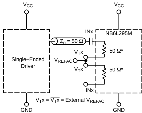
Figure 21. Capacitor-Coupled Single-Ended Interface ( V_{TX}/\sqrt{I_T X} Connected to External V_{REFAC} ; V_{REFAC} Bypassed to Ground with 0.1 \mu F Capacitor)
