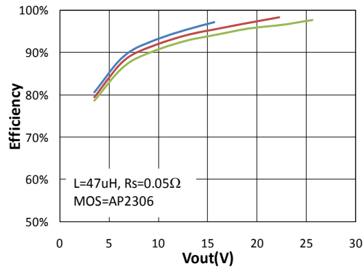
Efficiency vs. Output Voltage
