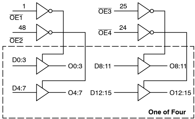
Figure 2. Logic Diagram
