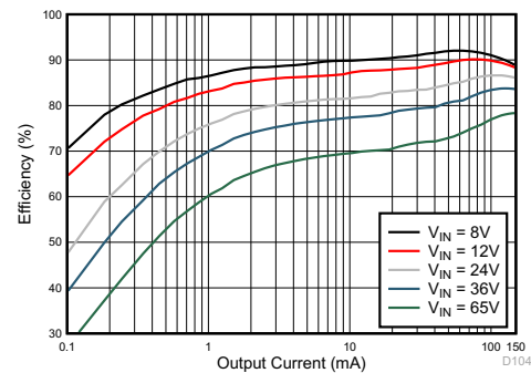
Figure 6-2. Converter Efficiency: 5 V, 150 mA, COT
