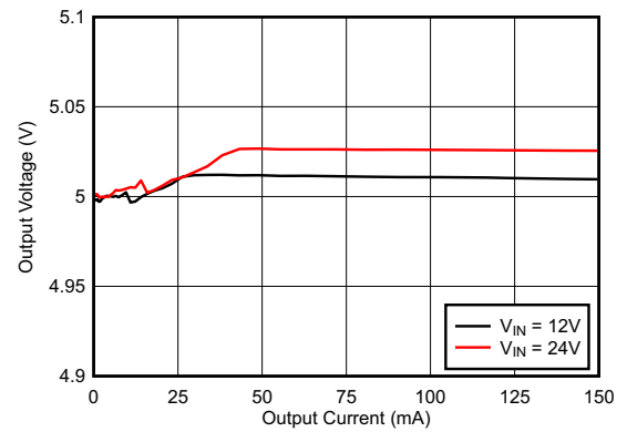
Figure 8-3. Load Regulation
