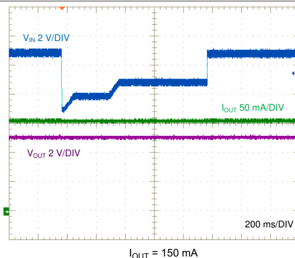
Figure 8-13. Input Transient (Automotive Cold Crank Profile)
