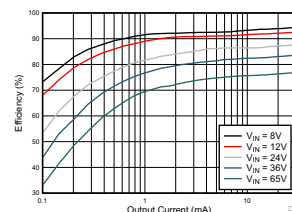
Typical Efficiency, V OUT = 5 V
