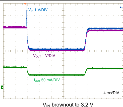
Figure 8-10. Dropout Performance, 75-mA Resistive Load
