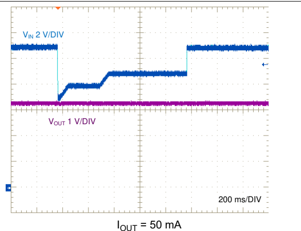
Figure 8-20. Input Voltage Transient (Automotive Cold Crank Profile)
