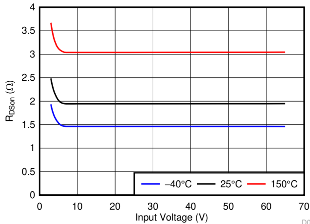
Figure 6-7. High-Side MOSFET On-State Resistance vs Input Voltage
