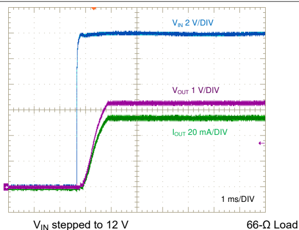
Figure 8-17. Start-Up, Full Load
