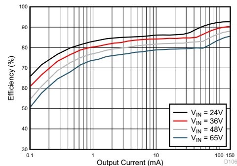
Figure 6-4. Converter Efficiency: 3.3 V, 150 mA, COT
