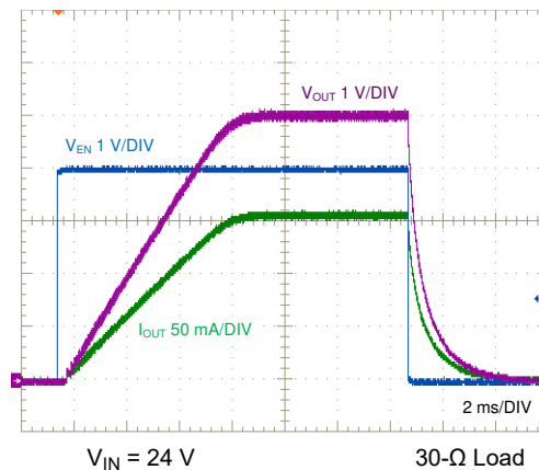
Figure 8-9. Enable ON and OFF
