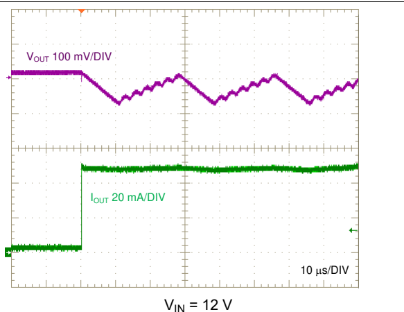
Figure 8-19. Load Transient, 0 mA to 50 mA, 1 A/ \mu\text{s}
