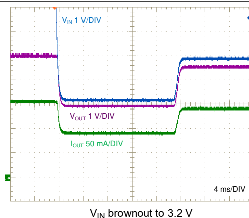
Figure 8-11. Dropout Performance, 150-mA Resistive Load
