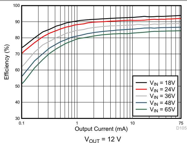
Figure 8-22. Efficiency
