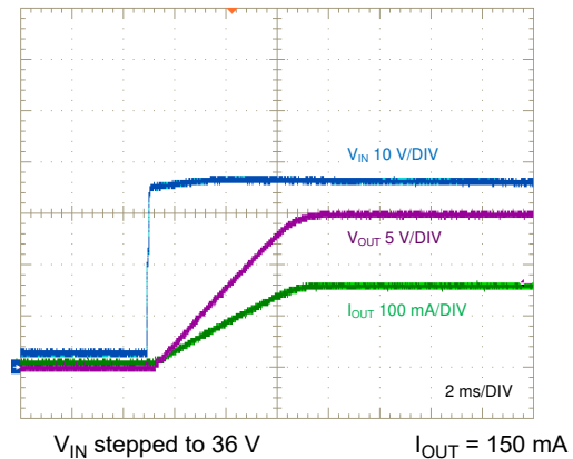
Figure 8-31. Start-Up, Full Load
