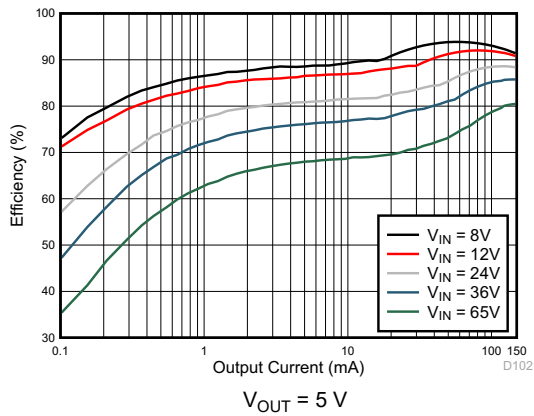
Figure 8-2. Efficiency
