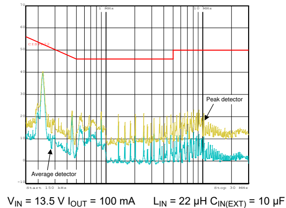
Figure 8-4. EMI Plot – CISPR 22 Filtered Emissions
