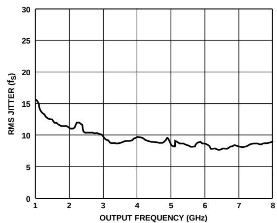
Figure 17. RMS Jitter vs. Output Frequency
