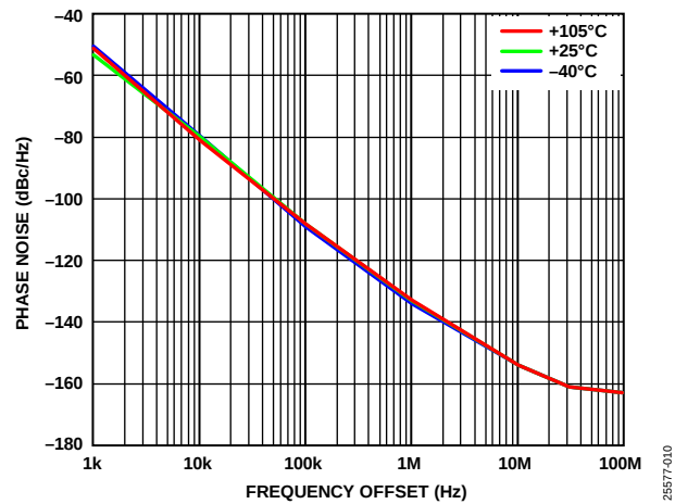
Figure 10. Open-Loop VCO Phase Noise over Temperature, 8.0 GHz, VCC_VCO = 5 V
