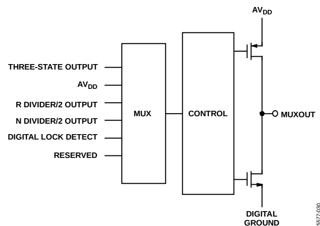
Figure 29. MUXOUT Schematic
