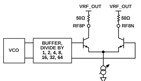
Figure 31. Output Stage
