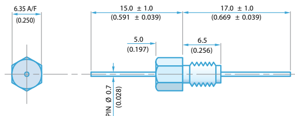
M5 x 0.8 - 6g Thread 6.35mm Hexagonal Head
