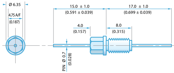
M5 x 0.8 - 6g Thread 4.75mm Hexagonal Head/6.35mm flange
