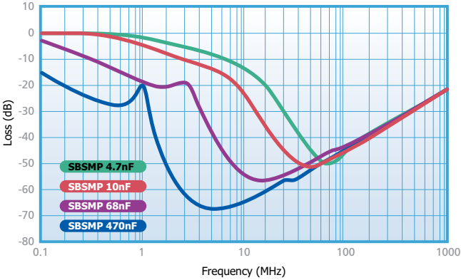
SBSMP Insertion Loss
