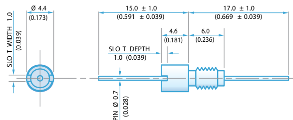
M3.5 x 0.5 - 6g Thread 4.4mm Round Head
