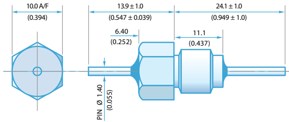
M8 x 0.75 - 6g Thread 10mm Hexagonal Head
