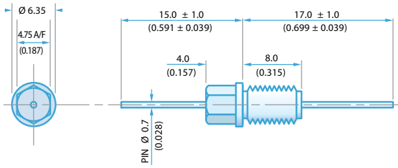
12-32 UNEF Class 2A Thread 4.75mm Hexagonal Head/6.35mm flange
