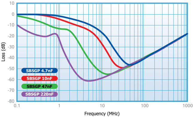
SBSGP Insertion Loss
