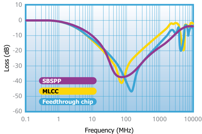
Comparison of 3.3nF SM filter types
