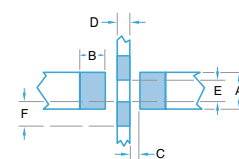
Recommended solder lands
