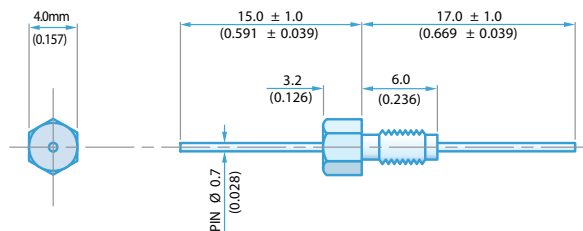
M3.5 x 0.6 - 6g Thread 4.0mm Hexagonal Head
