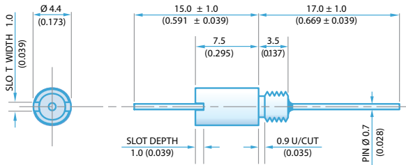
M3.5 x 0.6 - 6g Thread 4.4mm Round Head
