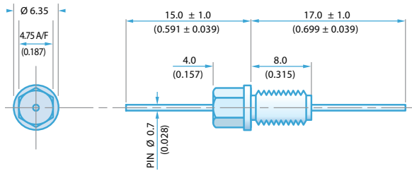
M5 x 0.8 - 6g Thread 4.75mm Hexagonal Head/6.35mm flange
