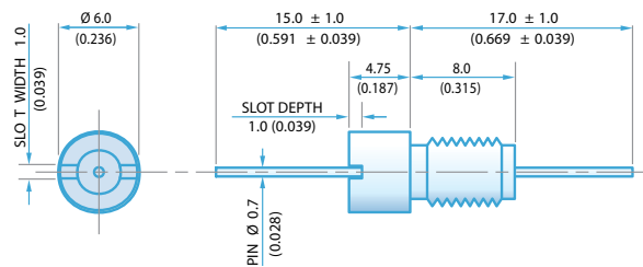
M5 x 0.8 - 6g Thread 6.0mm Round Head
