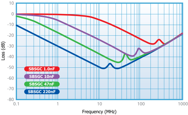
SBSGC Insertion Loss
