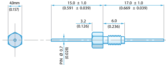
4-40 UNC Class 2A Thread 4.0mm Hexagonal Head
