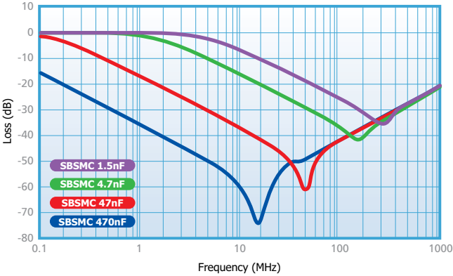
SBSMC Insertion Loss
