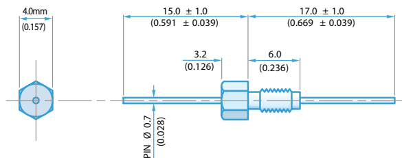
6-32 UNC Class 2A Thread 4.0mm Hexagonal Head
