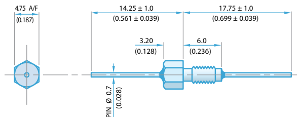
M4 x 0.7 - 6g Thread 4.75mm Hexagonal Head
