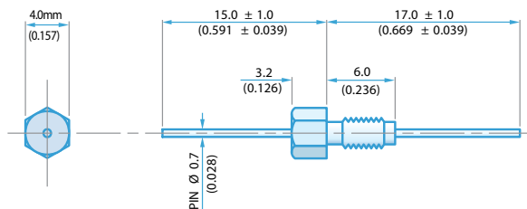
M3 x 0.5 - 6g Thread 4.0mm Hexagonal Head
