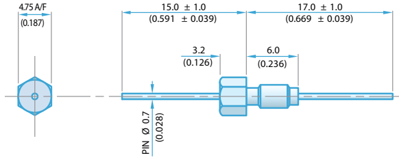
8-32 UNC Class 2A Thread 4.75mm Hexagonal Head
