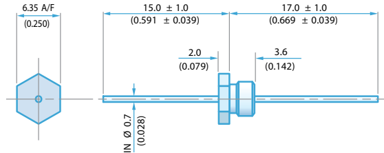
Low Profile M5 x 0.8 - 6g Thread 6.35mm Hexagonal Head
