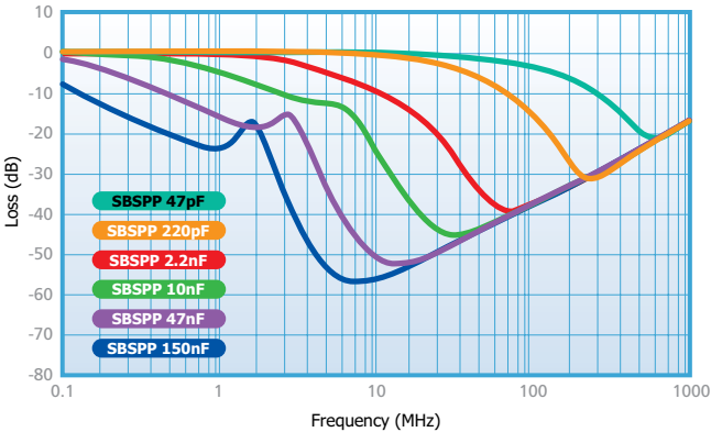
SBSPP Insertion Loss
