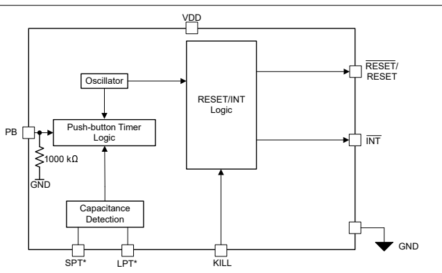
Figure 7-4. TPS3424 Block Diagram (Active High Push-Button Input)
