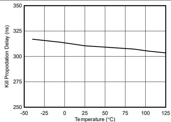
Figure 6-13. Kill Propagation Delay vs Temperature
