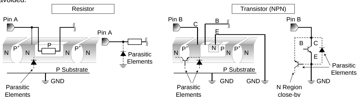
Appendix: Example of monolithic IC structure
