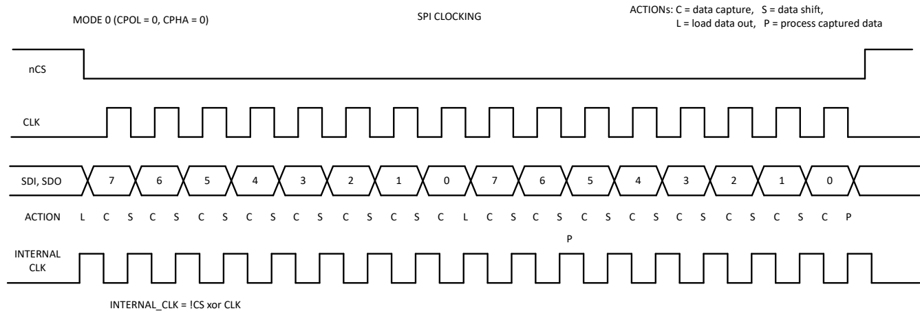
Figure 8-54. SPI Clocking
