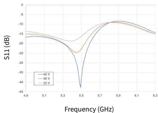
Figure 42. Input RL vs Frequency as a Function of Voltage
