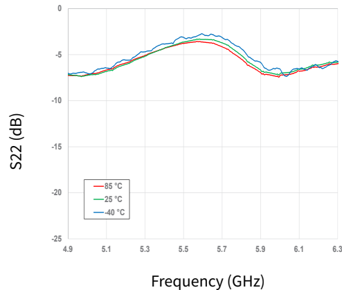
Figure 39. Output RL vs Frequency as a Function of Temperature
