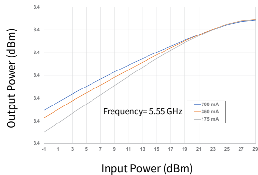
Figure 23. Output Power vs Input Power as a Function of I_{DQ}
