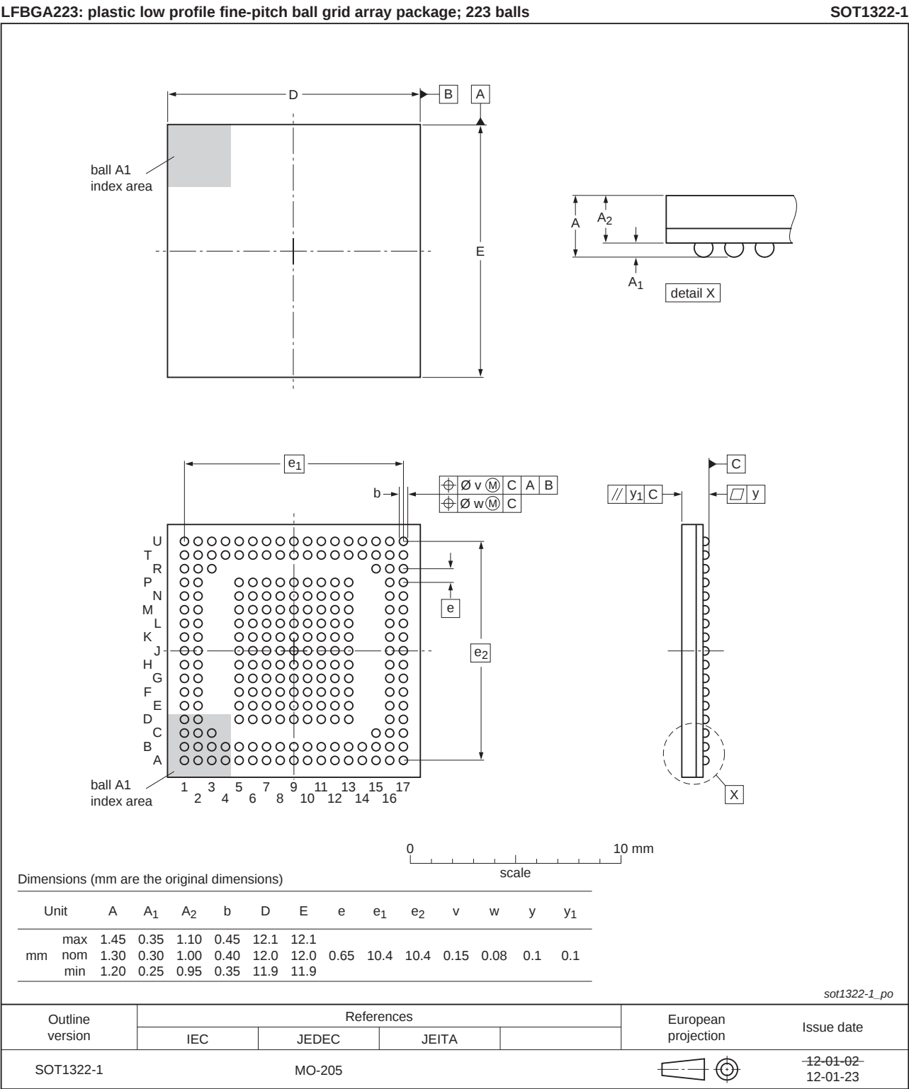
Fig 5. Package outline SOT1322-1 (LFBGA223)
