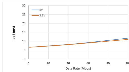
Figure 17. Si88243 Typical V_{ddb} Supply Current vs. Data Rate (5 and 3.3 V Operation)
