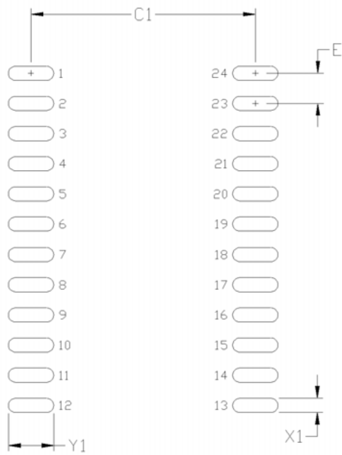
Figure 38. 24-Pin SOIC PCB Land Pattern
