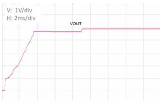
Figure 25. 5 V–5 V VOUT Startup vs.Time (No Load)
