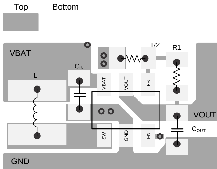
Figure 30. PCB Layout
