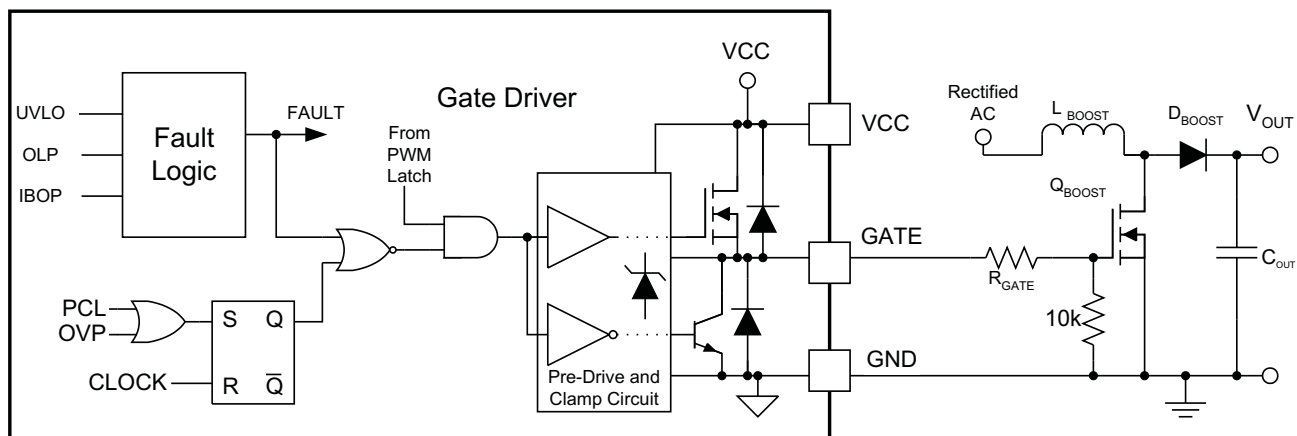
Figure 24. Gate Driver
