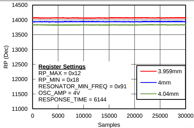
Figure 2. R_p Resolution
