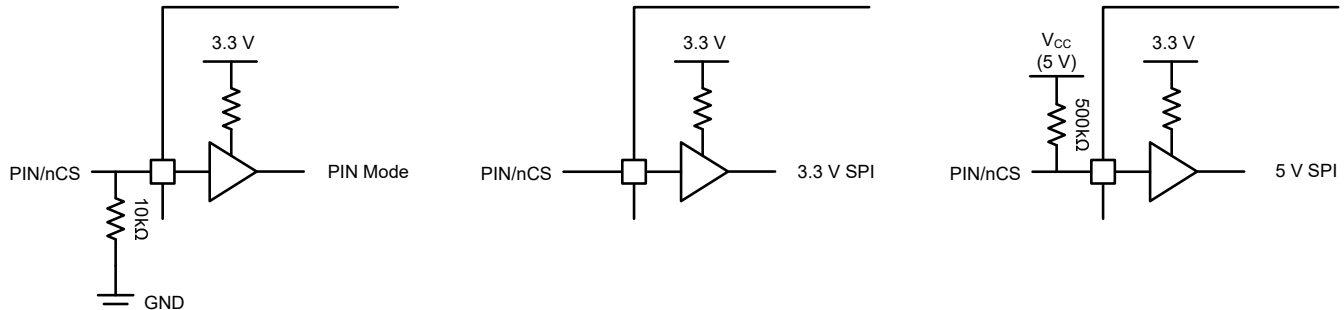
Figure 8-4. PIN/nCS configuration
