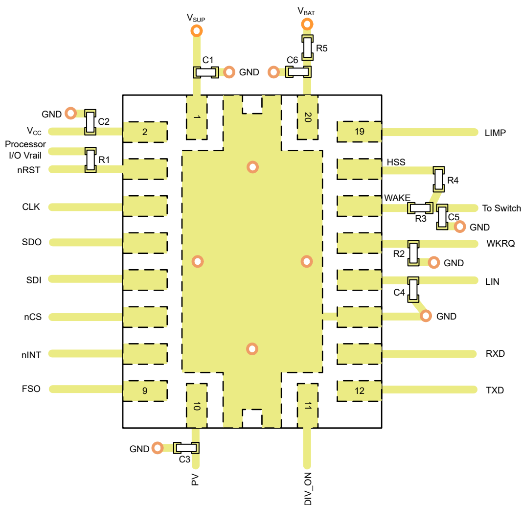
Figure 9-14. Layout Example
