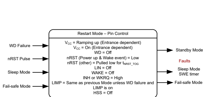
Figure 8-38. Restart Mode Pin Control
