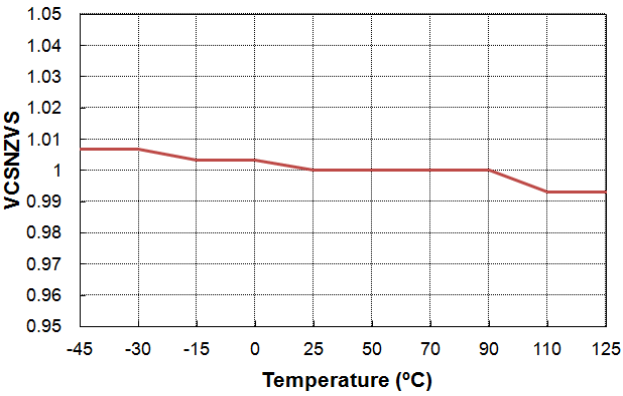
Figure 51. VCS.NZVS vs. Temperature
